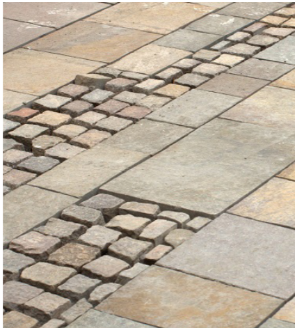
Paving design as 'overlapping carpets' - matching stone type but with varying unit size, finish, laying pattern and direction.
