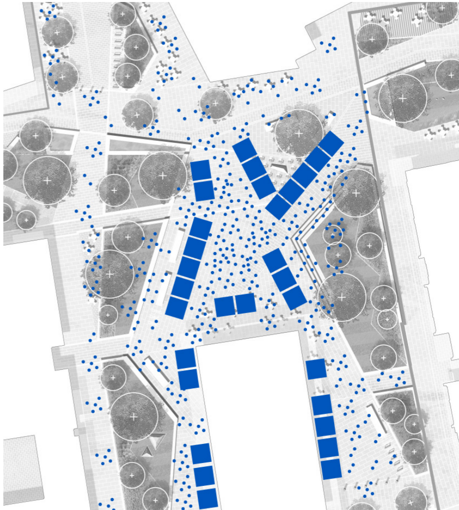
Events use - farmers market - 30no. 3x3m stalls and 500 people shown
