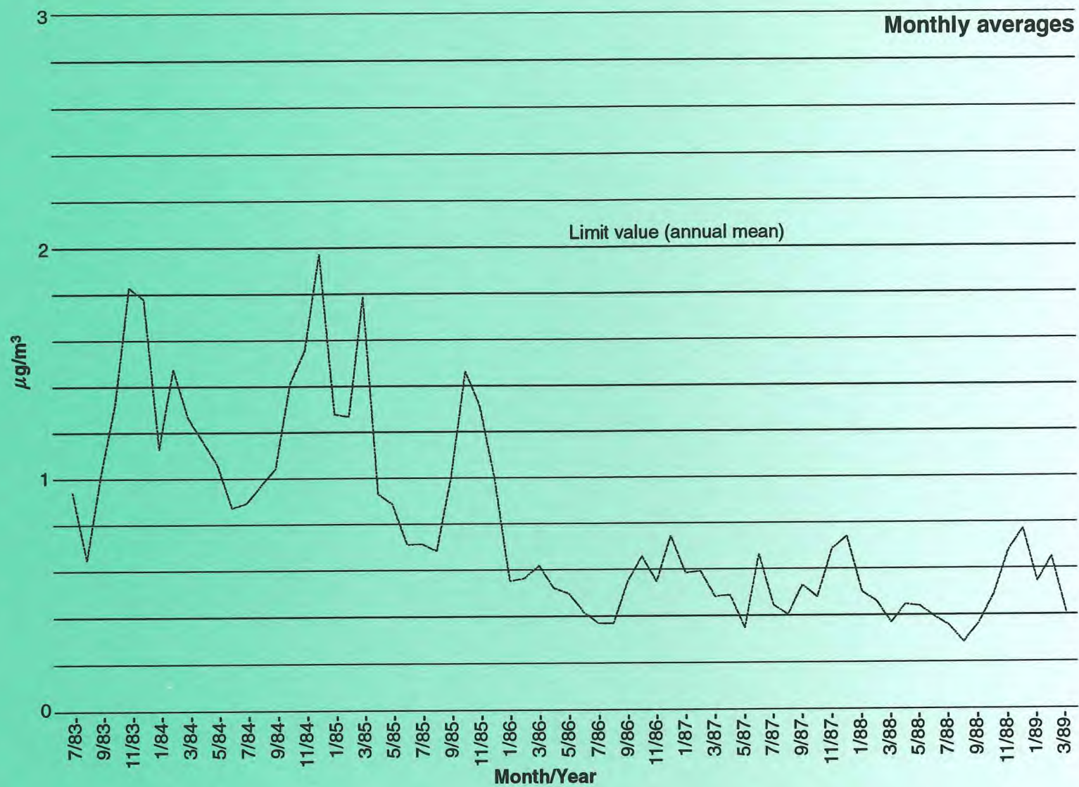
Figure 5.9 Lead levels at Evelina Road July 1983 to March 1989
